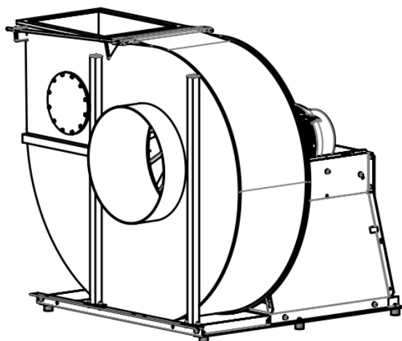
Vibration damper for floor mounting
