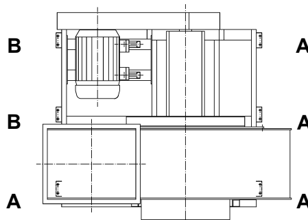
V-belt drive
