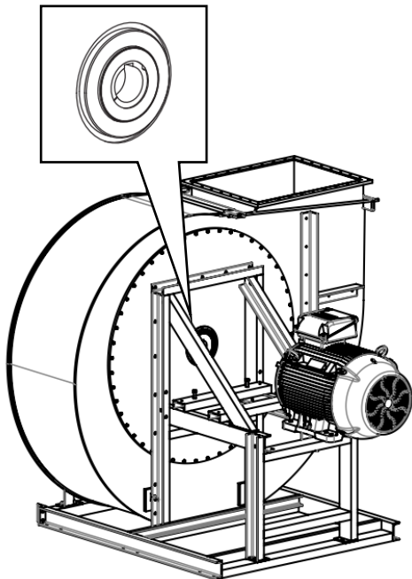
Single lip seal
