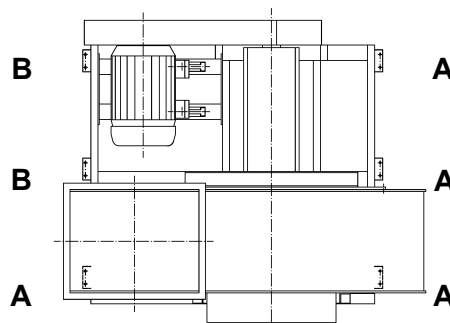
V-belt drive
