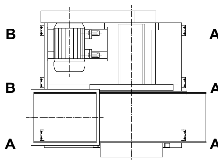
V-belt drive
